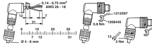
Functional drawing
